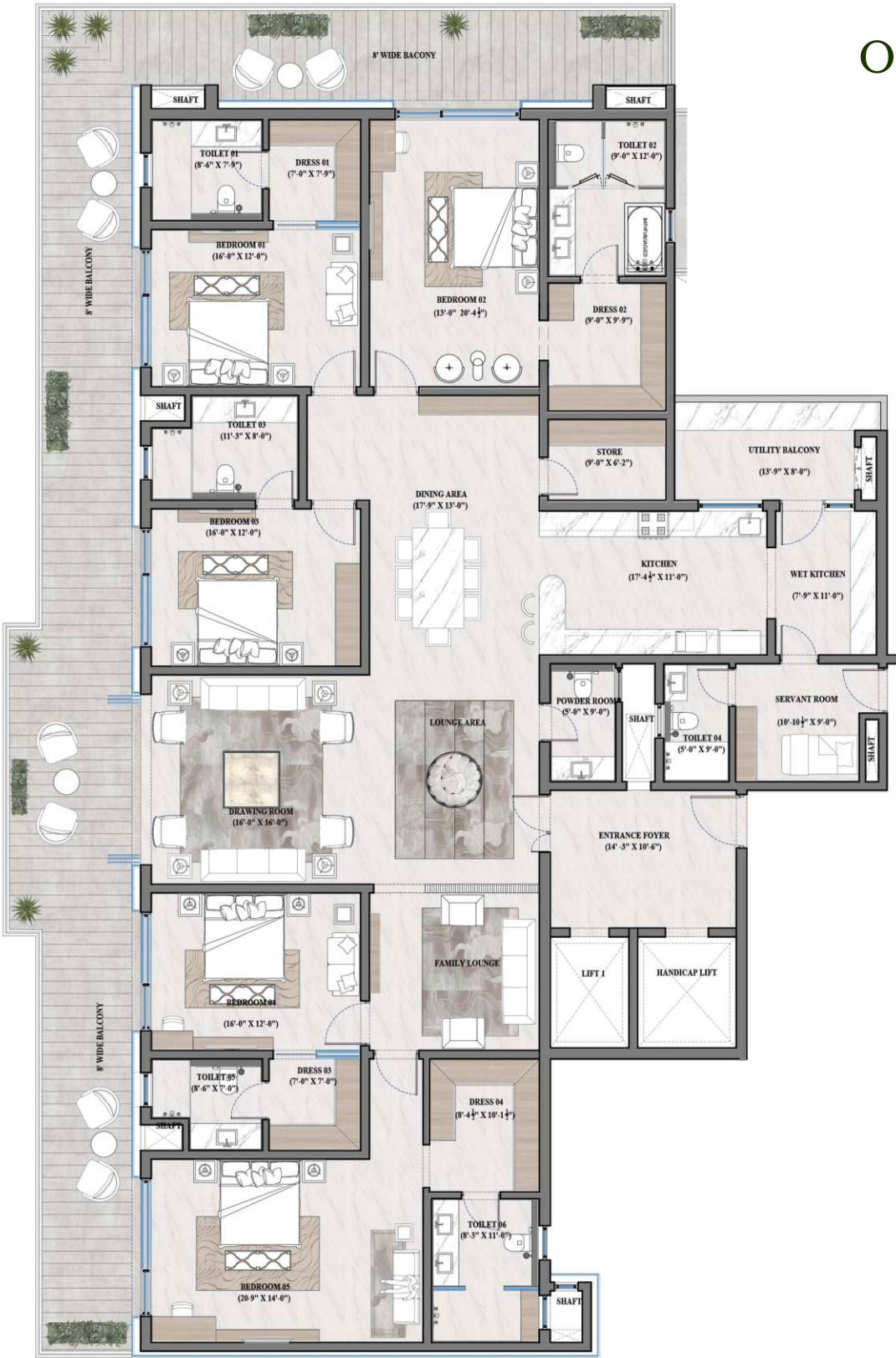
ZENELIA HOUSE TYPICAL UNIT PLAN - 5+1 BHK (UNIT-1)
